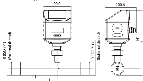
S 421 thread type
